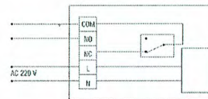
Type A: Voltage-free output wiring diagram
