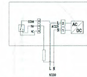
Type B: 230V output wiring diagram
