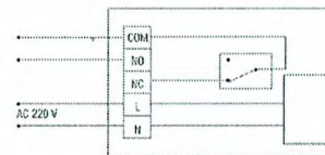
Type A: Voltage-free output wiring diagram
